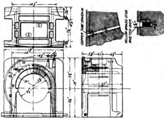
Figs. 1405-1409. Cast-Steel Driving Box for Journals 9½ in. x 13 in. Atlantic (4-4-2) Locomotive. Pennsylvania Railroad.
